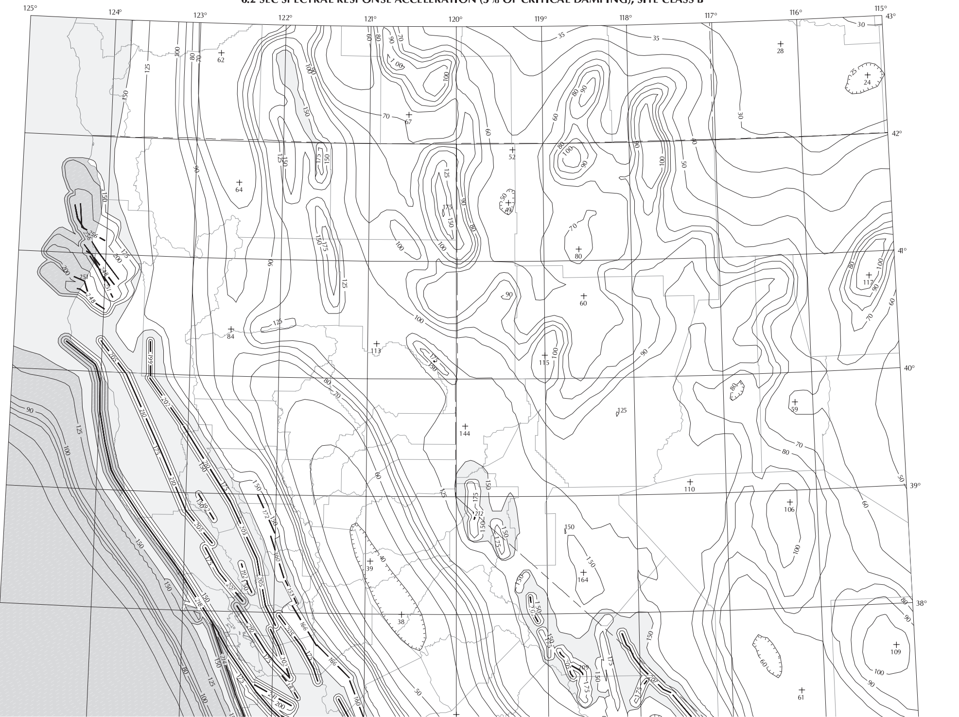
FIGURE 1615 (3) MAXIMUM CONSIDERED EARTHQUAKE GROUND MOTION FOR REGION 1 OF 0.2 SEC SPECTRAL RESPONSE ACCELERATION (5% OF CRITICAL DAMPING), SITE CLASS B
